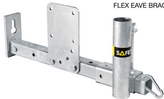
FLEX EAVE BRACKET
